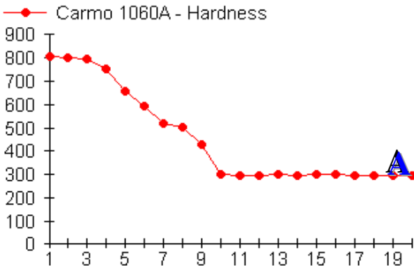
Hardness vs Depth Carmo
