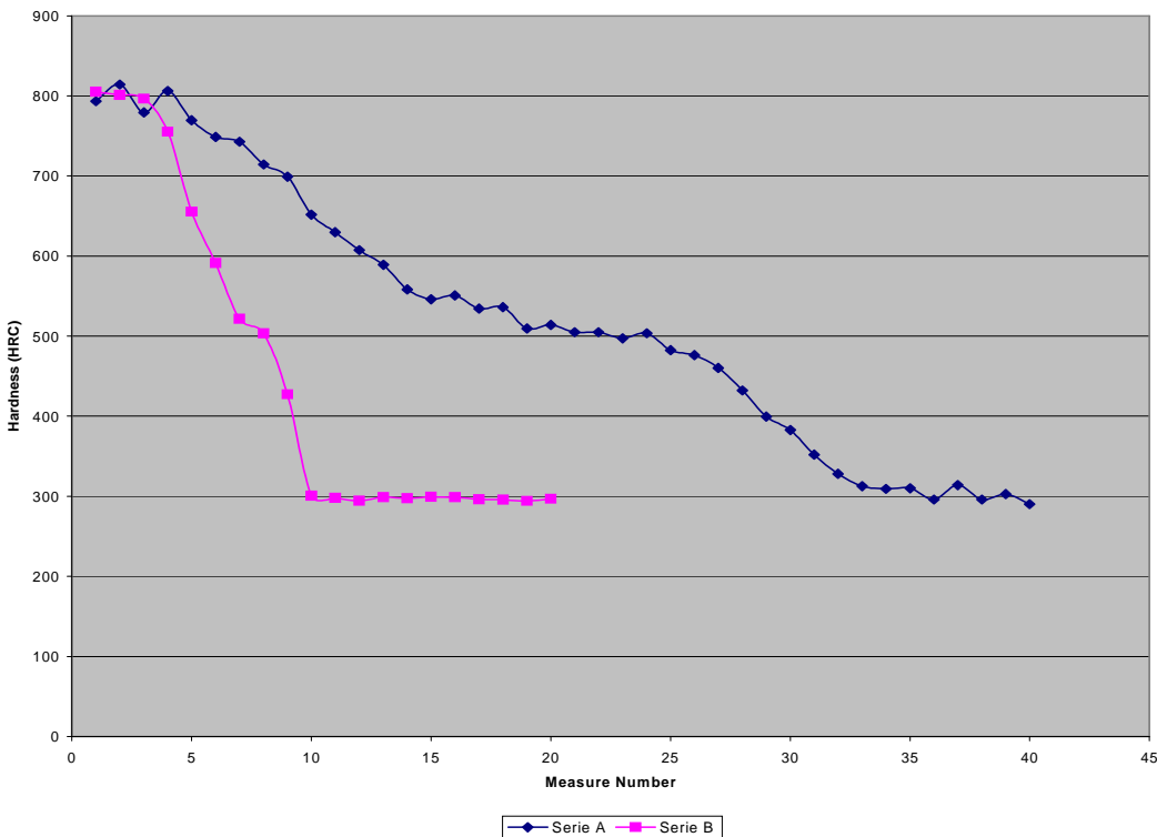
Hardness vs Depth Carmo
